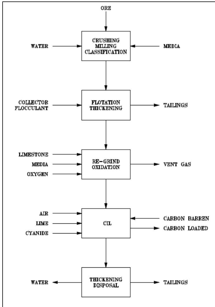
Figure 8: Albion Outline Process Flow Diagram (Ref. 18: Xstrata/Core/Aker Paper at Randol Forum Perth 2005)
