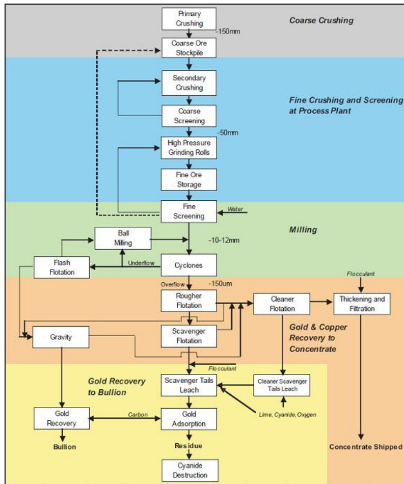
Figure 1: Boddington Expansion Flowsheet (Ref. 3: Newmont/Boddington Gold Paper at World Gold 2007)
