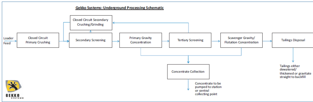
Figure 3: Gekko Underground Processing (Python) Flowsheet (Ref. 5: Gekko/Central Rand Gold Paper at First International Future Mines Conference 2008)
