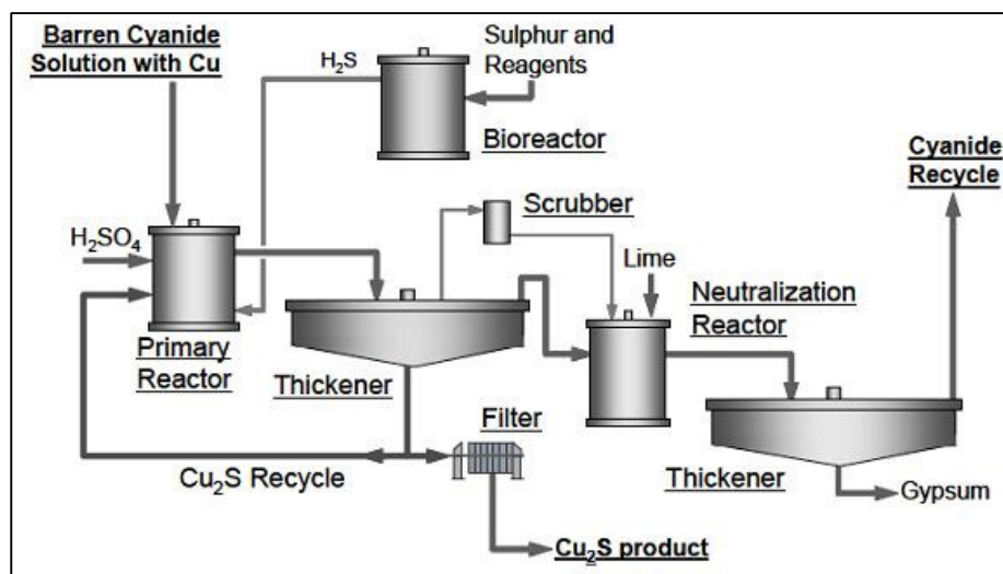
Figure 6: Bioteq BioSulphide Process Flowsheet (Ref. 8: BioteQ Paper at Precious Metals 07)
