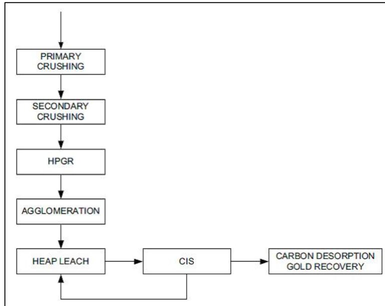
Figure 2: HPGR Heap Leach Flowsheet (Ref. 4: Orway Paper at HR Crushing & Grinding 2006)
