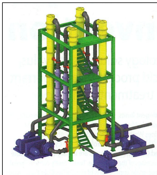
Figure 7: Schematic of MMS Archen Reactors and Leach Columns (Ref. 17: Mining Magazine Jan./Feb. 2010)
