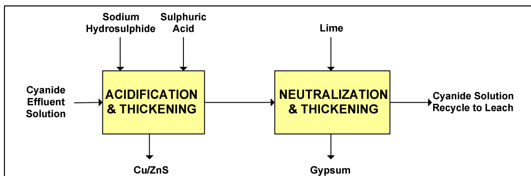
Figure 5: Simplified SART Flowsheet
