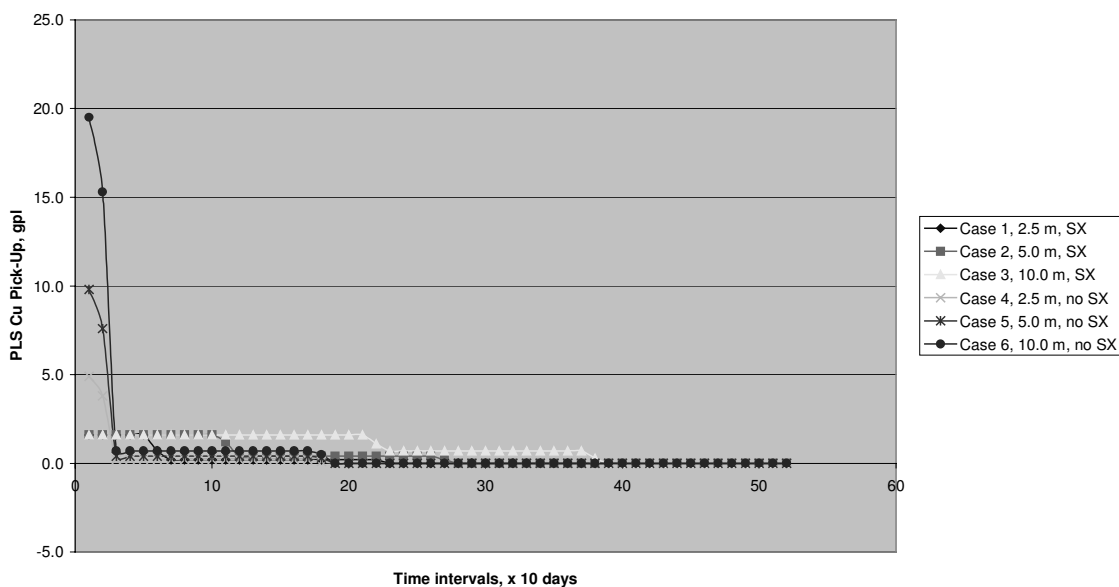
Fig 4.5: PLS Cu Pick-Up vs Time: Heap Heights 2.5-10m, with SX Constraint and with no SX constraint
