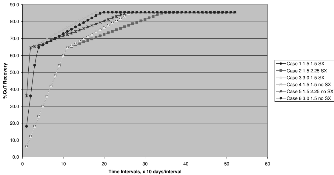
Fig 4.5 – PLS Cu Pick-up versus Time: Variable Heap Height and SX Constraint
