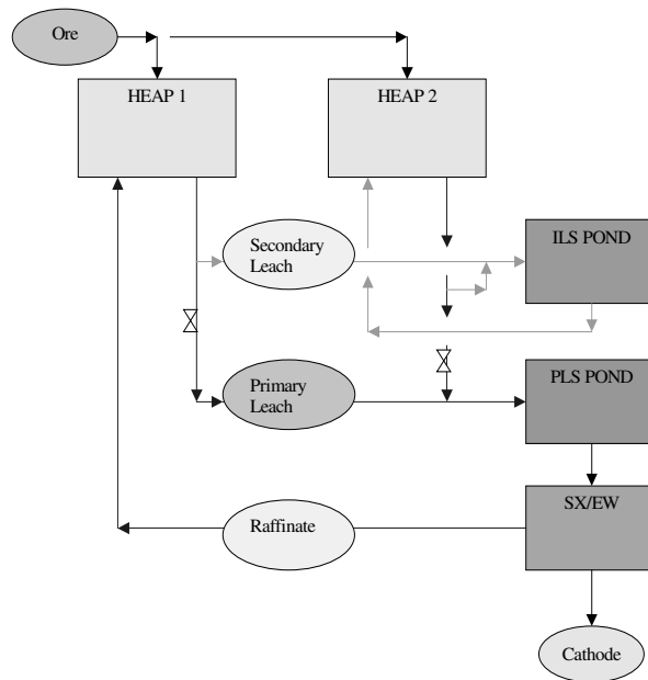
Fig 1: Multiple Heap or Fixed Heap Leach System
