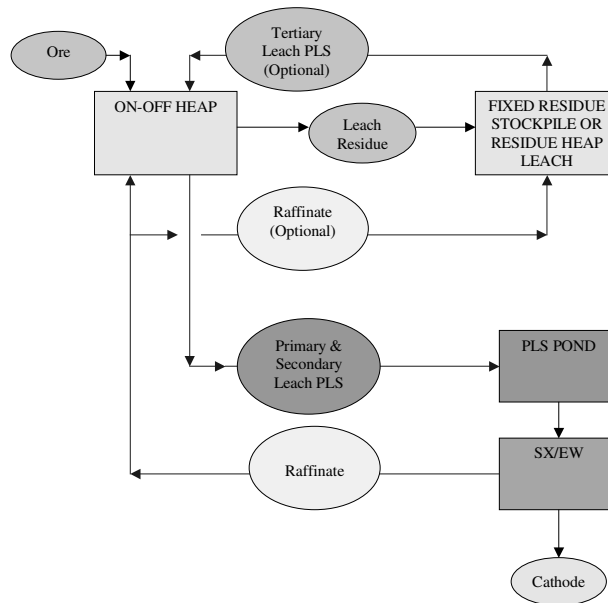
Fig 2: Single Heap On-Off Re-useable Pad Leach
