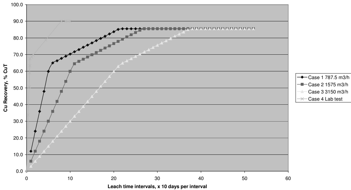
Fig 4.2: % CuT Recovery vs Leach Time Intervals for Lab Test and Varying PLS Flow Rates
