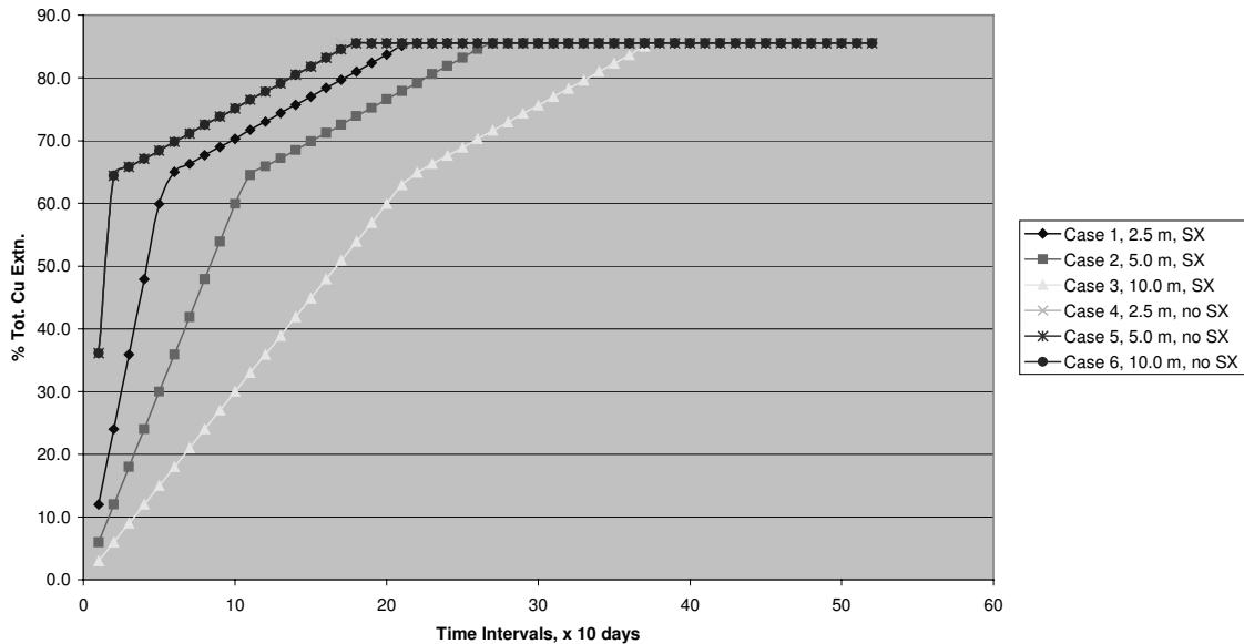
Fig 4.6: % Tot. Cu Extn. versus time: Heap Heights 2.5-10m, with SX constraint and with no SX Constraint
