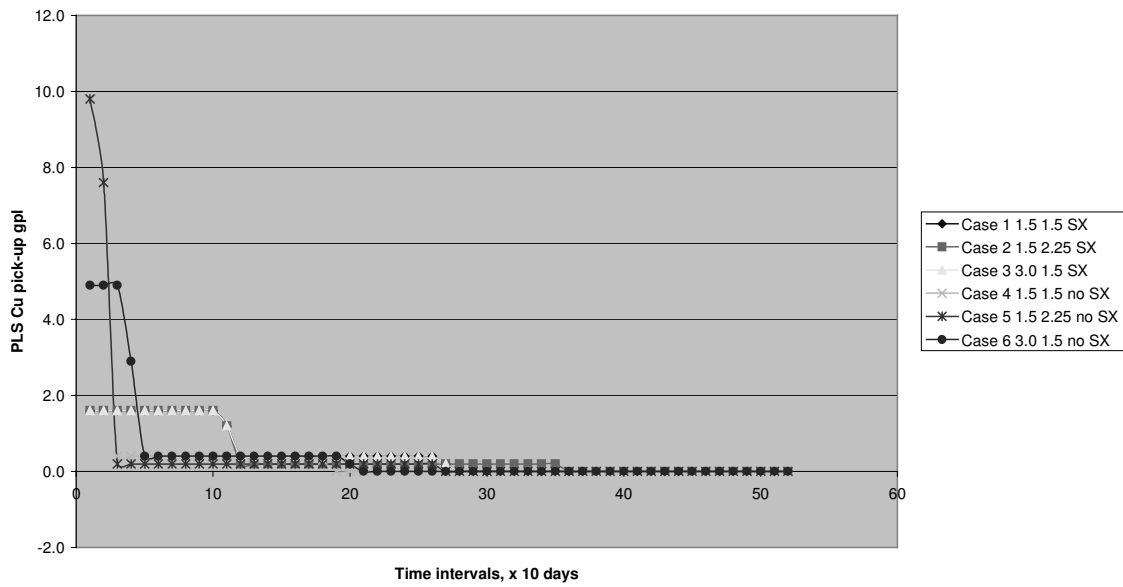
Fig 4.3: PLS Cu Pick-up vs Time: Primary and Secondary Safety Factors 1.5 - 3, with SX constraint and with no SX constraint
