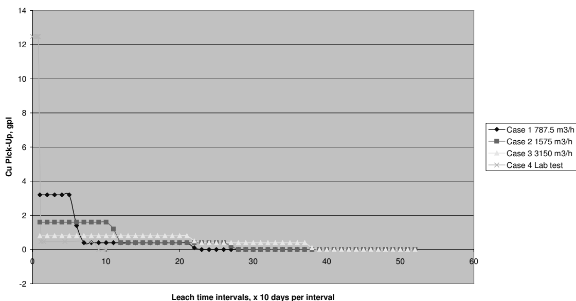
Fig 4.1: PLS Cu Pick-up vs Leach Time Intervals for Lab Test and Varying PLS Flow Rates
